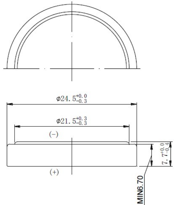
Dimension Drawing
